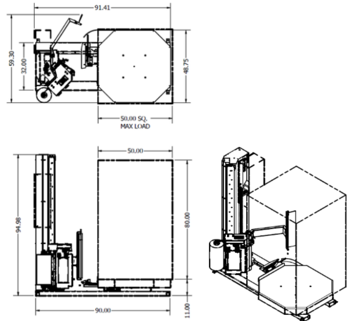
Flex HPA - Dimensions - Inches
