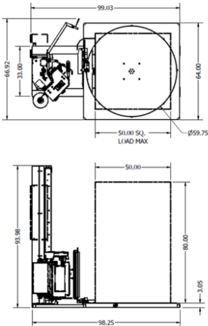
Flex LPA - Dimensions - Inches
