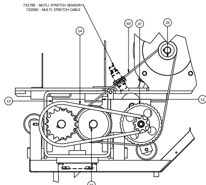
DETAIL A SCALE 3/8
