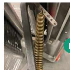
Adjustable dancer bar and spring options allow fine tuning of tension
