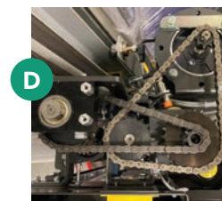
Heavy duty chain drive and gear ensure consistent performance
