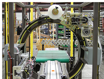
Orbital bridge and film carriage
